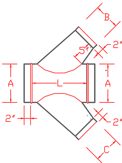
CLC45 CONICAL LATERAL CROSS 45° L = \text{Largest Tap} \times 1.414 + 5"
