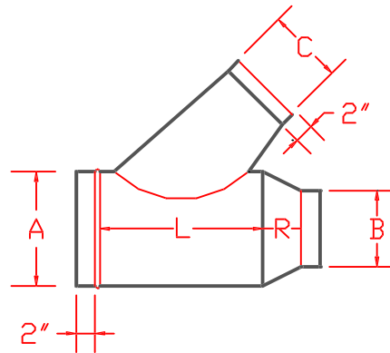
CRL45 CONICAL REDUCING LATERAL 45° L = C \times 1.414 + 5" R = Refer to reducer drawing.
