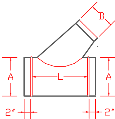
CL45 CONICAL LATERAL 45° L = B \times 1.414 + 5"
