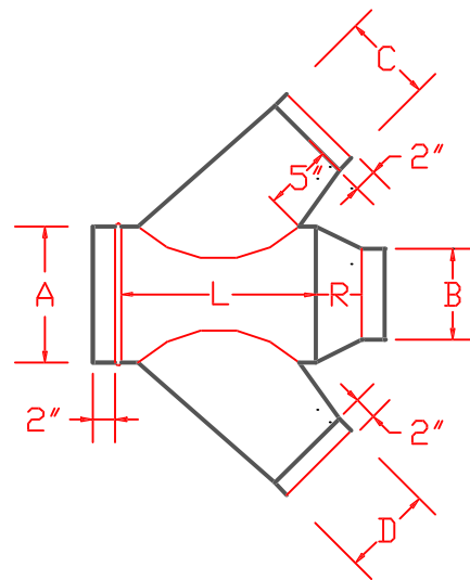
CRLC45 CONICAL REDUCING LATERAL CROSS 45° L = \text{Largest tap} \times 1.414 + 5" R = Refer to reducer drawing.
