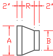
CR CONCENTRIC REDUCER
